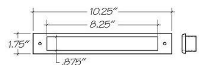
Slotted Outlet Dimensions
